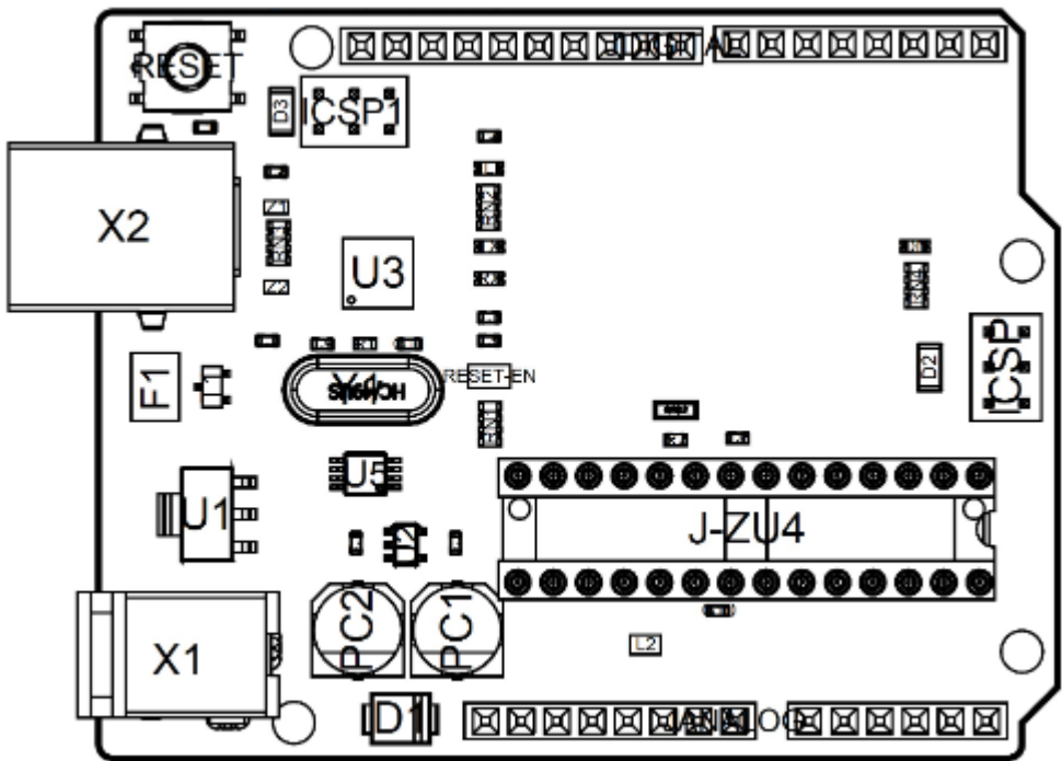
Board topology
